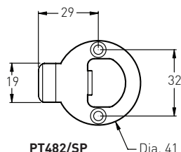
PT482/SP Drive-in Strike Plate
