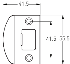
PT480/SPSQ Rectangular Strike Plate
