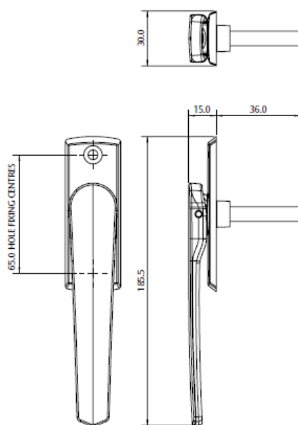
Aria Style Bi-fold Handle
